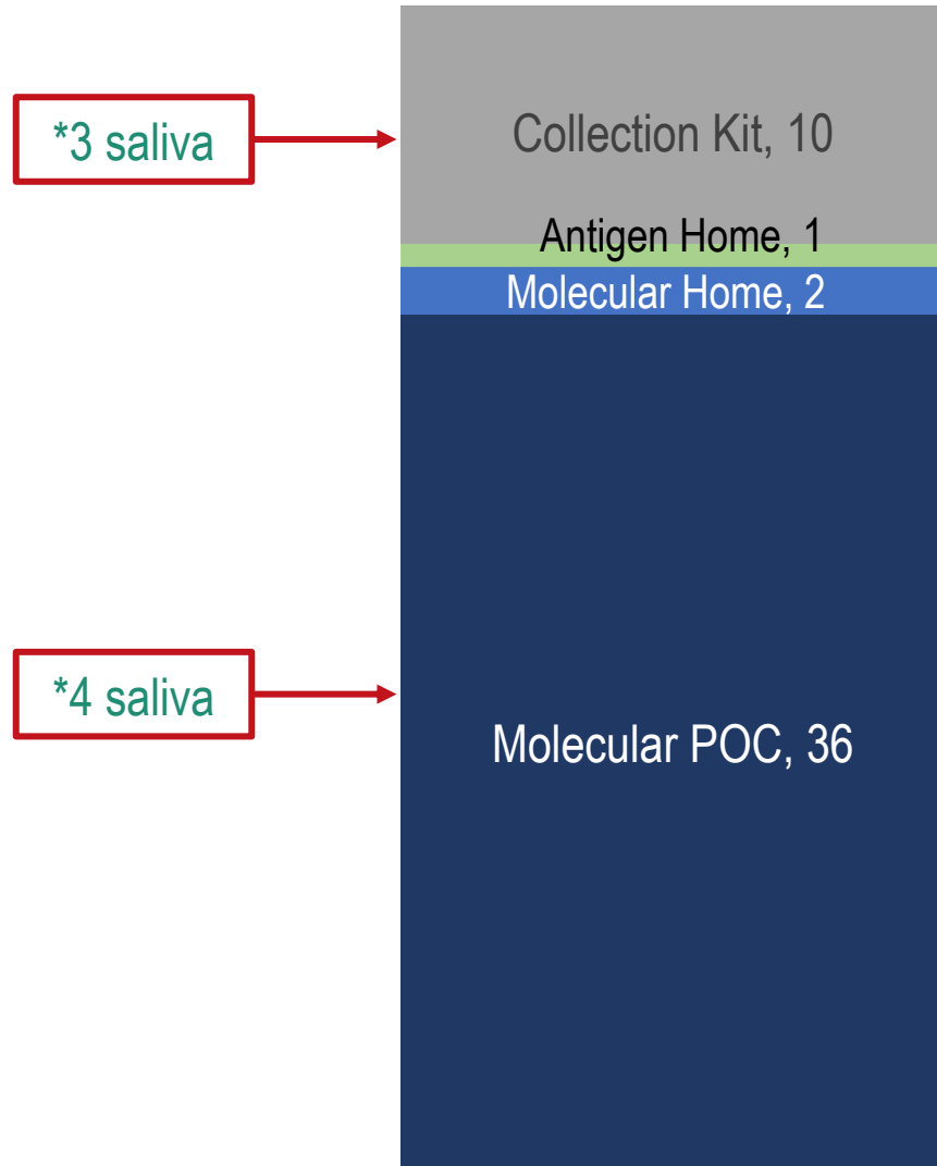
Screening (49)
