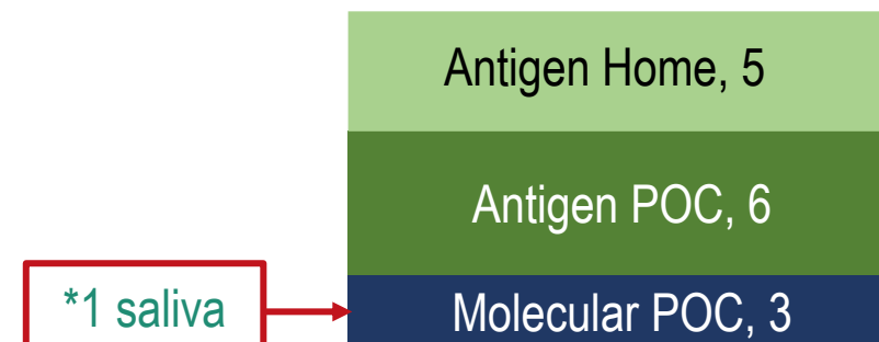
Serial Screening (14)
